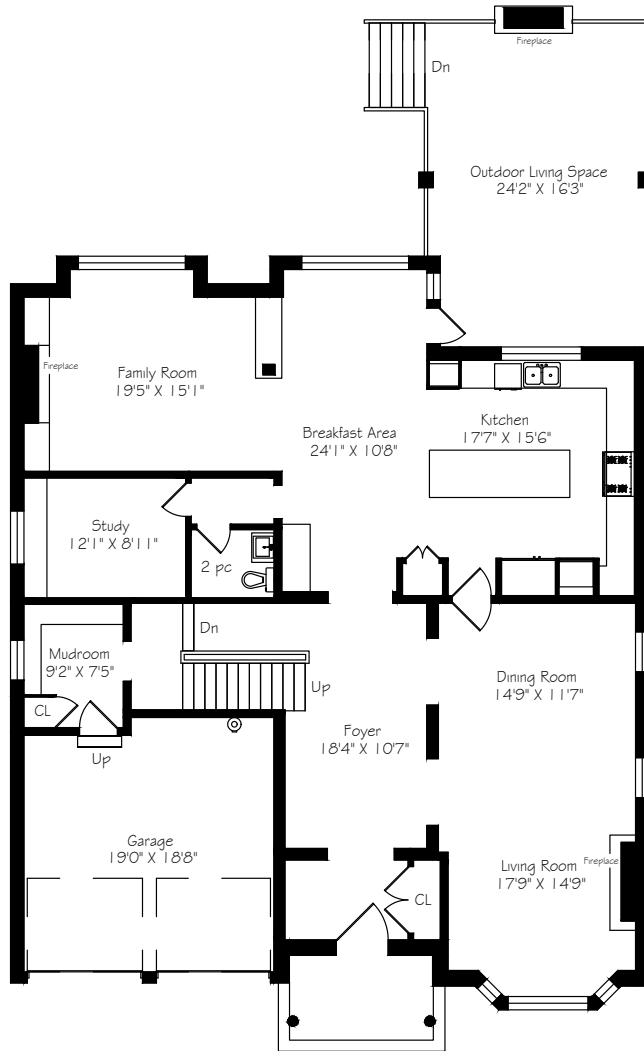
Main Floor 2090 Square Feet
