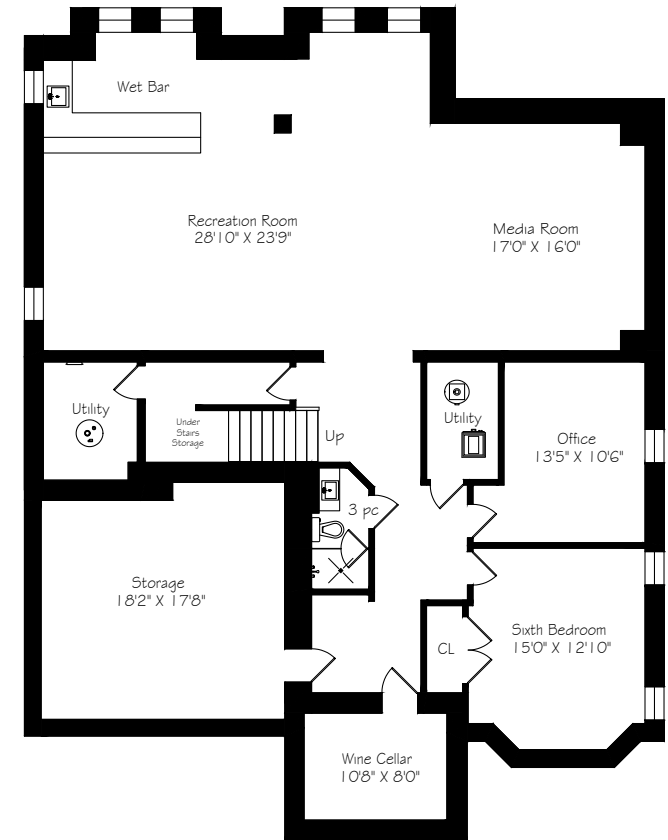
Lower Level 2478 Square Feet
