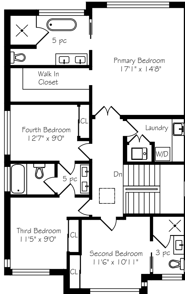
Second Floor 1312 Square Feet
